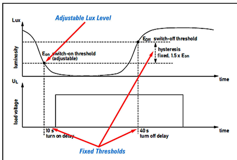
Switching Thresholds
